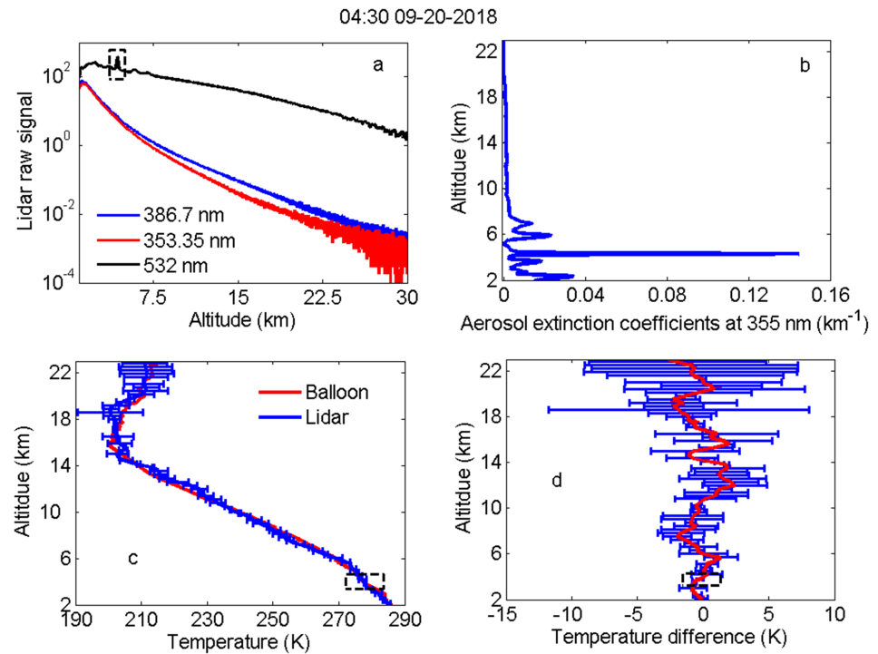
Figure 3. (a) HU lidar elastic (black), VR (blue line), and RR (red line) lidar signals; (b) aerosol extinction coefficients at 355 nm calculated using Raman technique; (c) temperature profiles obtained using the proposed technique (blue line) and radiosonde (red line); (d) temperature difference between the proposed technique and the local radiosonde launched in HU at 04:30 on 20 September 2018.
